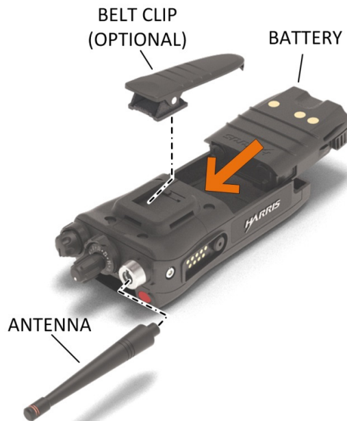
Figure 4-1: Radio Assembly
